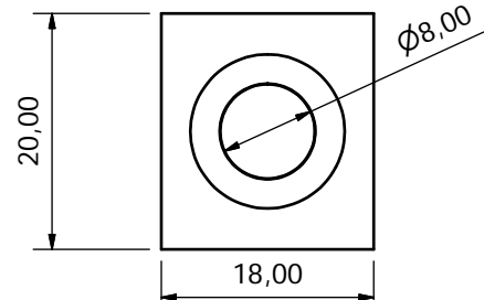
HC0820-18 23.80mm HIGH
